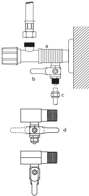
Figure 3. Water connection fittings
