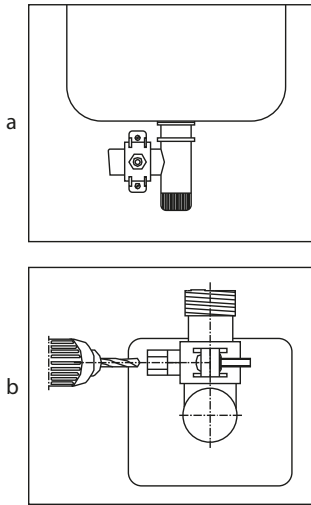
Figure 5. Waste water connection
