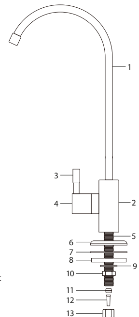
Figure 4. Faucet
