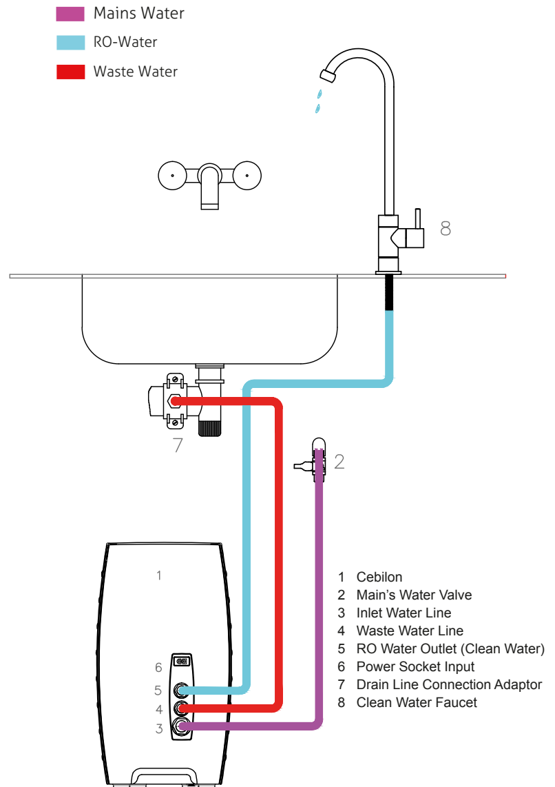
Figure 2. RO Installation Scheme
